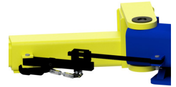
Automatic swing arm restraint
